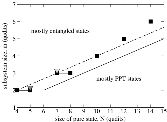
FIG. 2: Numerical results showing the transition from entangled to PPT subsystems. For each m , points are shown for which P_{\text{PPT}} \in (1\%, 99\%) for qubits (■) and qutrits (grey ▽). The solid/dashed lines represent the range in eq. (15).
