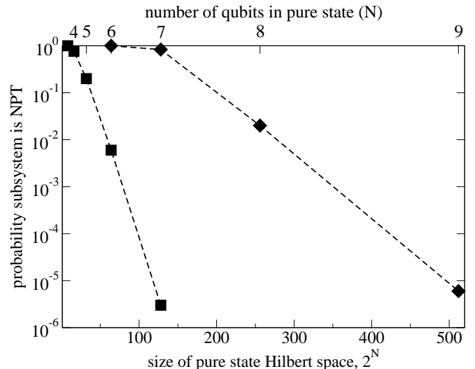
FIG. 3: Probability of finding that a subsystem of m qudits is entangled in random pure states sampled uniformly over the Haar measure for qubits for m = 2 (■) and m = 3 (filled ◇).
